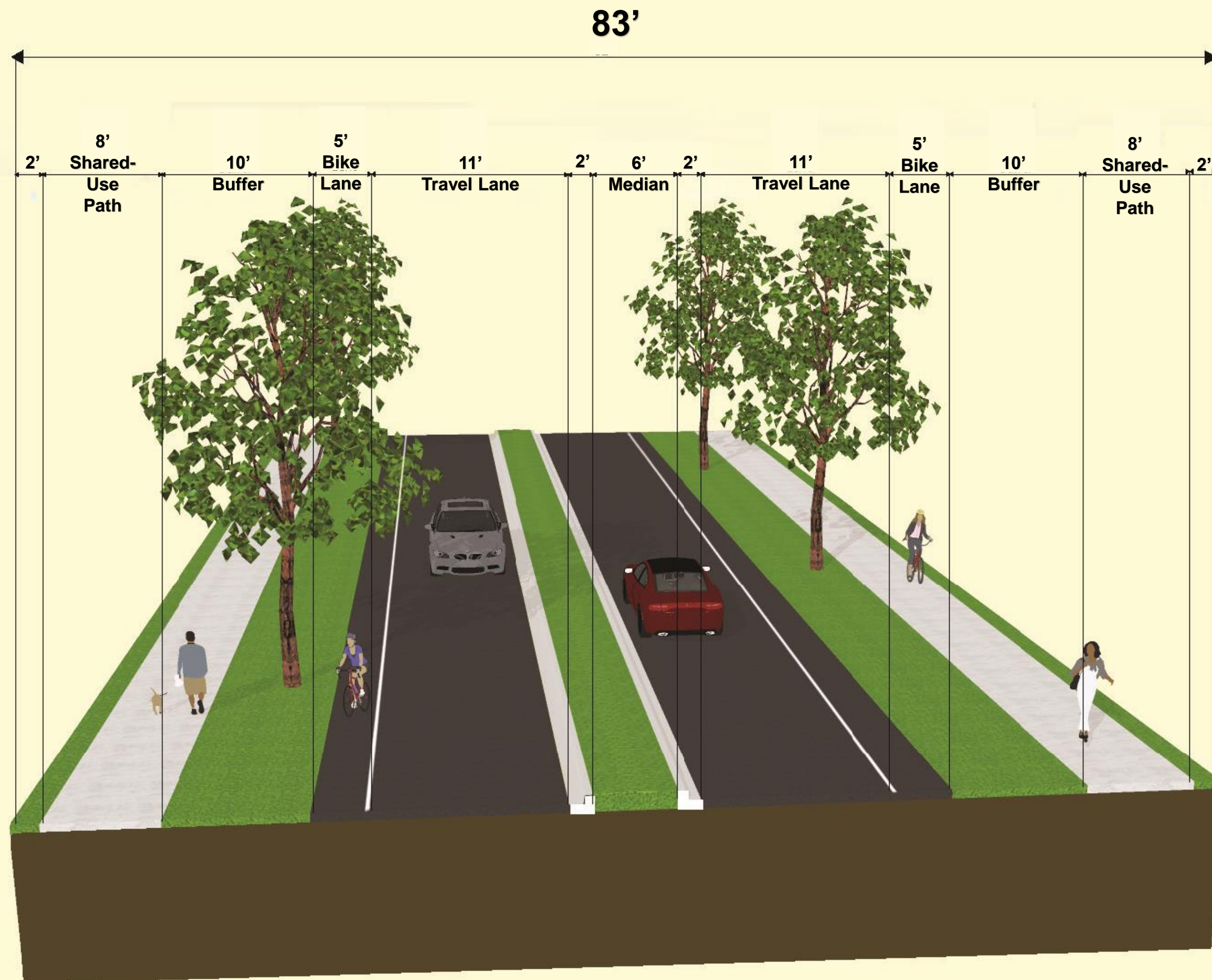
Alternative 1: Divided Roadway with Shared-Use Facility on Both Sides
