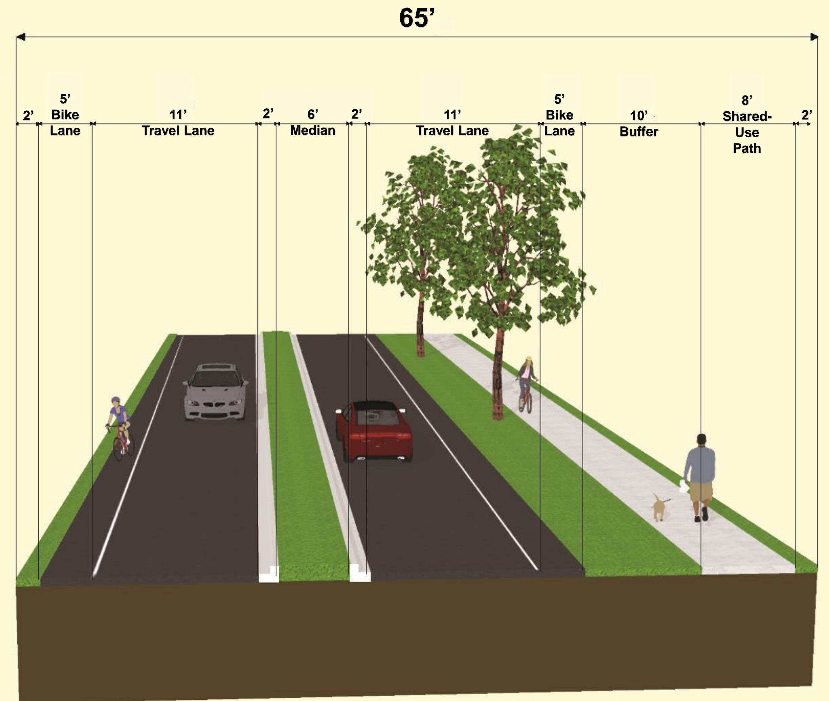
Alternative 2: Divided Roadway with Shared-Use Facility on Town Side
